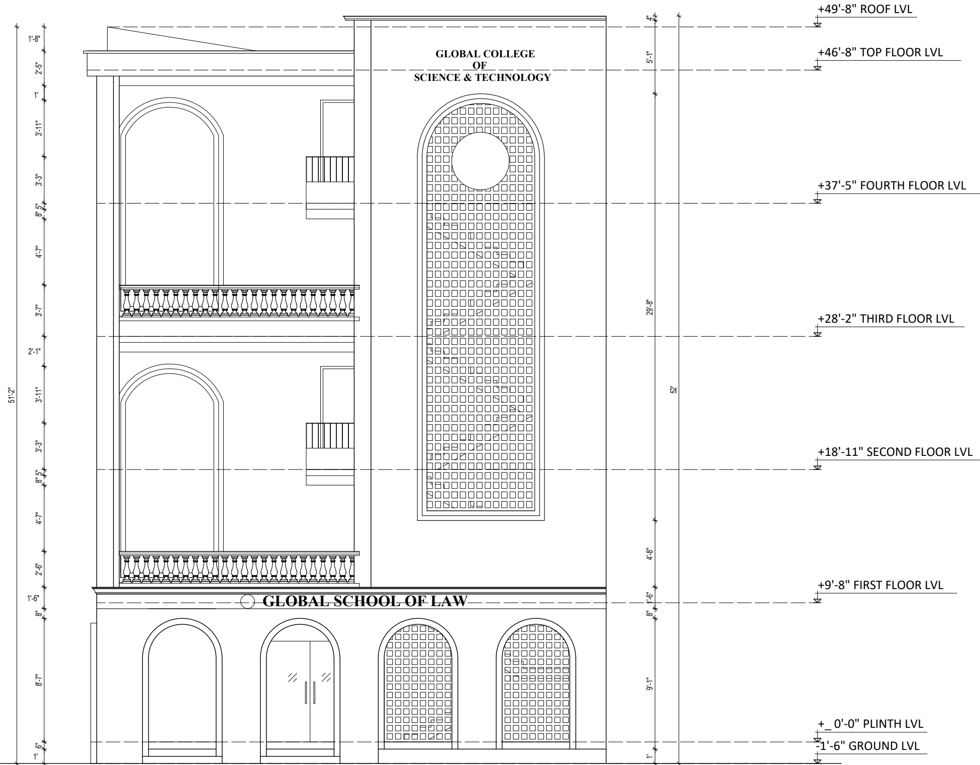
NORTH ELEVATION
