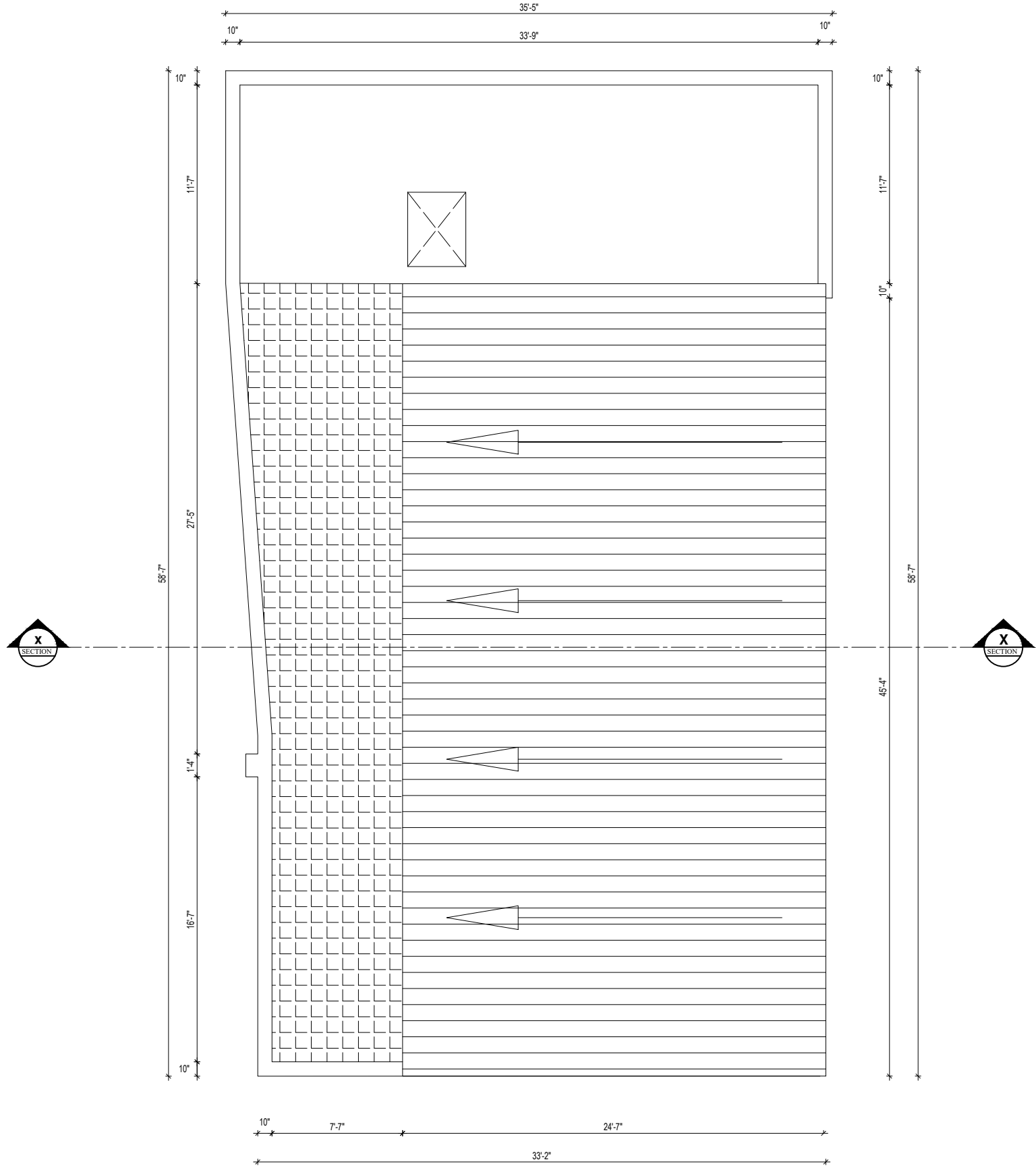
ROOF PLAN
