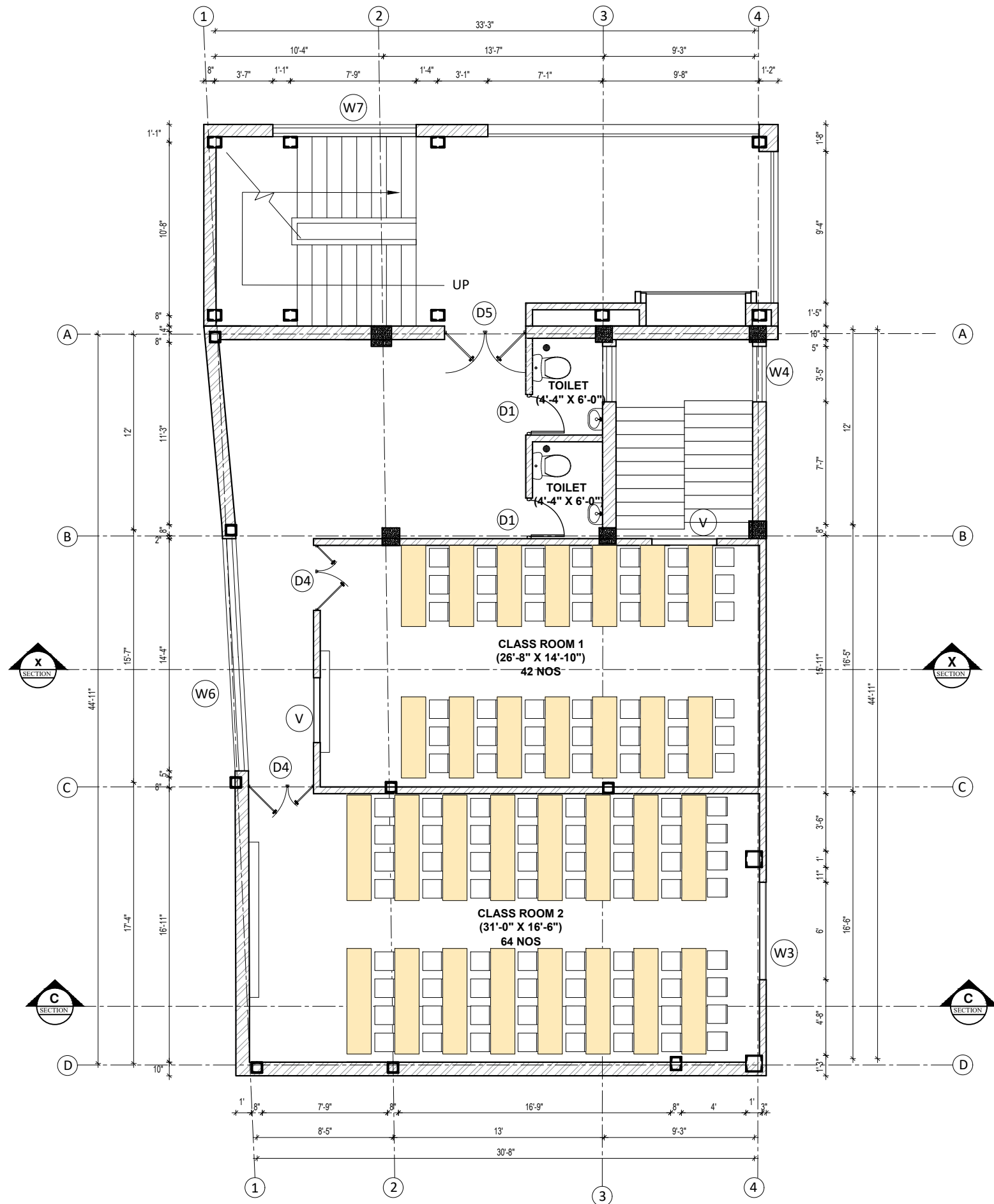
THIRD FLOOR PLAN AREA: 1975.02 SQ. FT.
