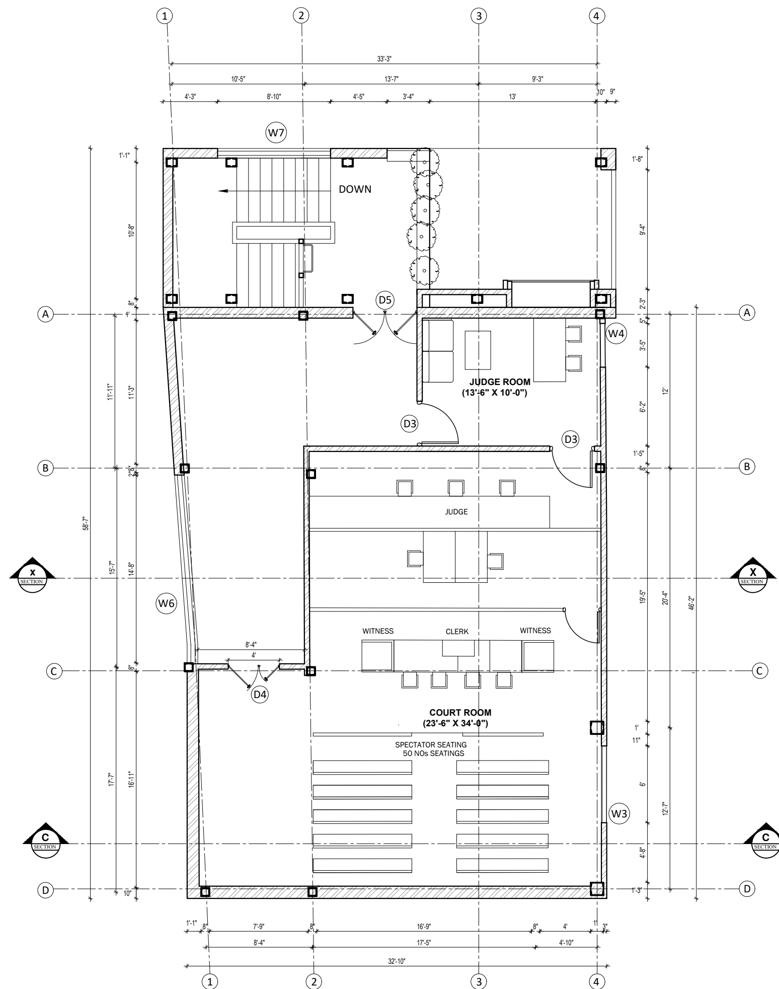
TOP FLOOR PLAN AREA: 1975.02 SQ. FT.
