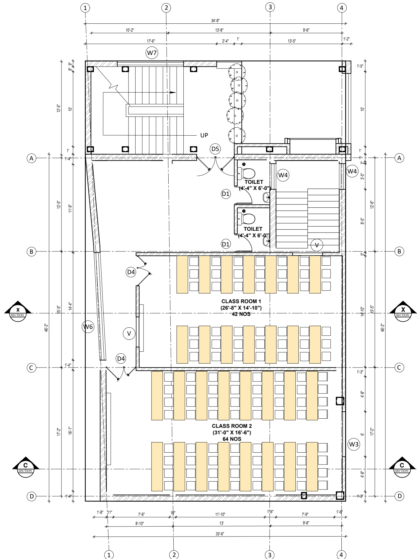
SECOND FLOOR PLAN AREA: 1975.02 SQ. FT.
