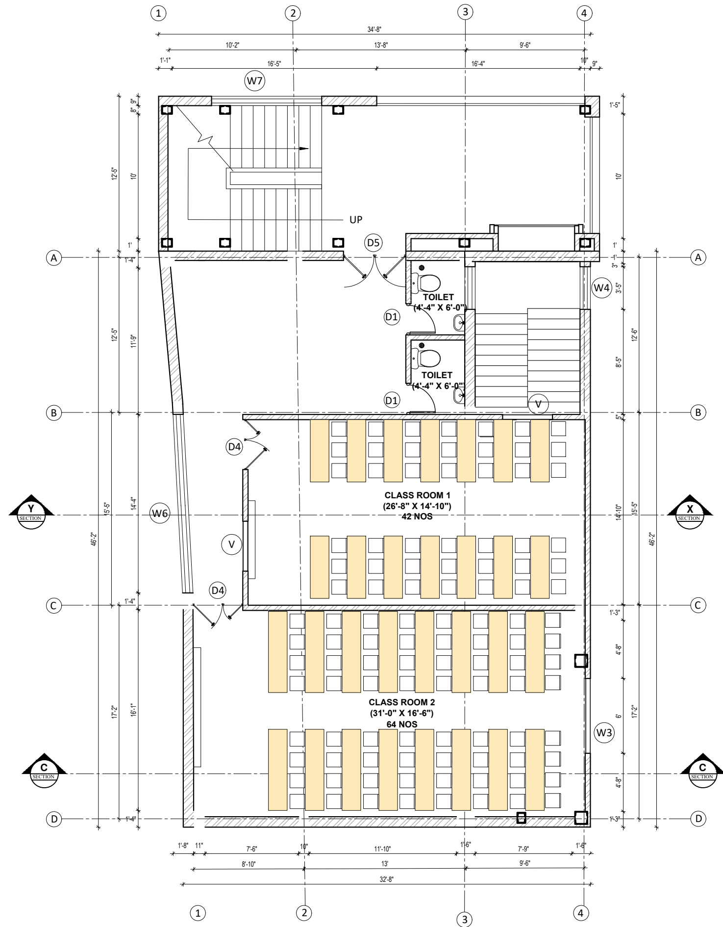
FIRST FLOOR PLAN AREA: 1975.02 SQ. FT.
