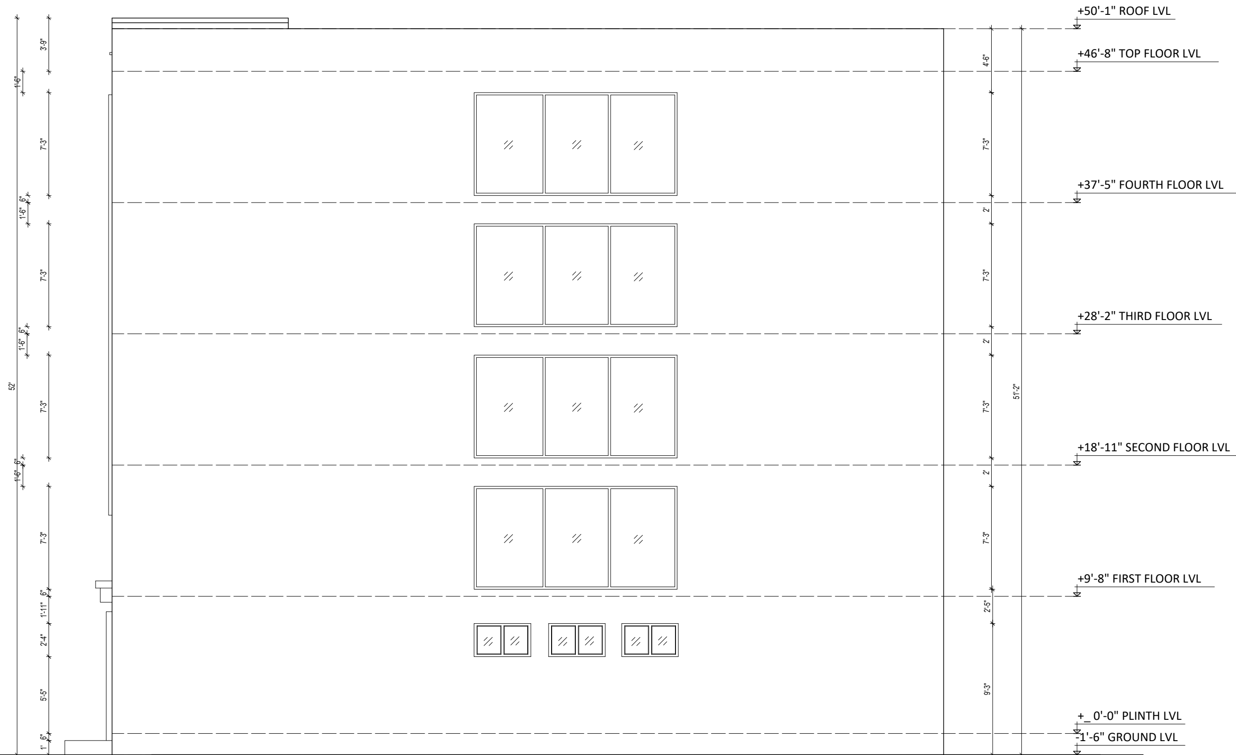
WEST ELEVATION
