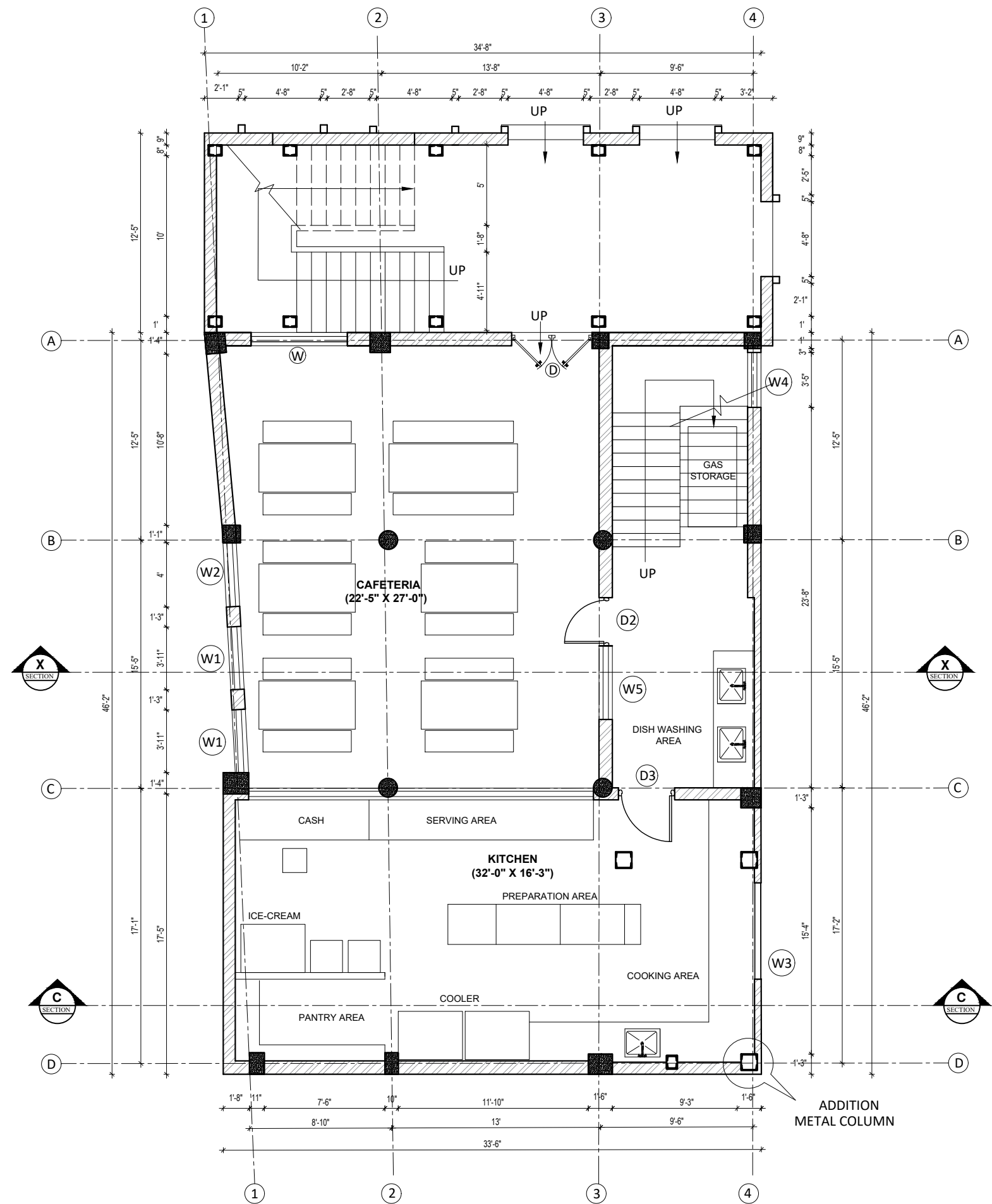
GROUND FLOOR PLAN AREA: 1988.18 SQ. FT.
